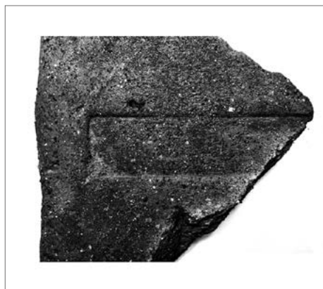
Fig. 10. Example of a stamp from the bathhouse excavation: fragment of a rectangular field with an almost illegible inscription C[---] (Gonio/Apsaros Project/photo K. Żywicki)
