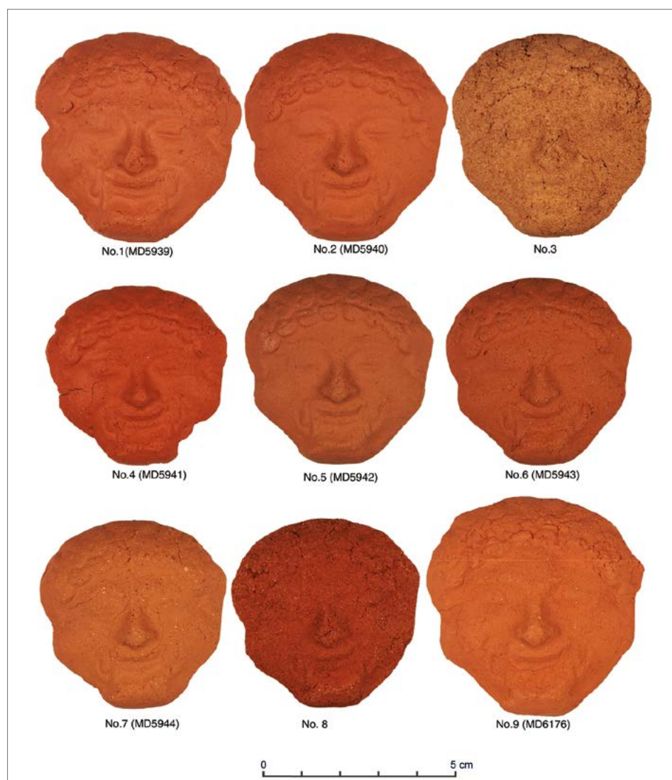
Fig. 15. Plasticity test: samples formed in plaster moulds and fired at 900°C in an oxidising atmosphere in a laboratory kiln (Digitizing M. Daszkiewicz, photos M. Baranowski)
